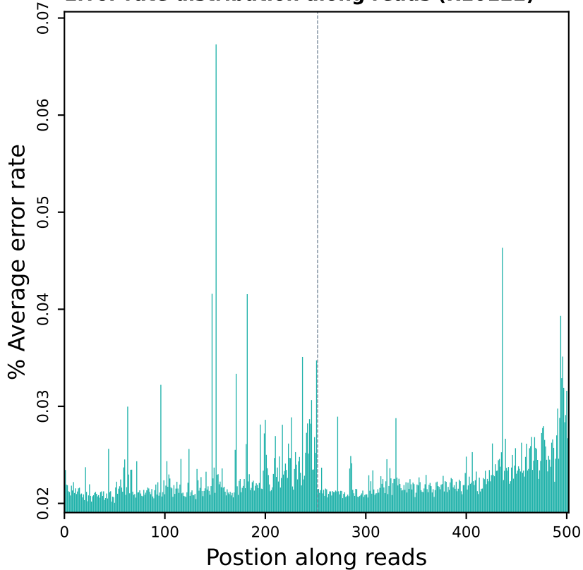
Error rate distribution along reads (R10122)
